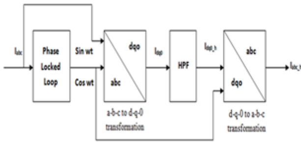
Fig. 3. Harmonic Extraction Block.
