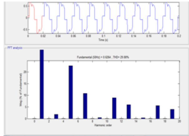
Fig. 11. FFT Analysis Before Compensation.
