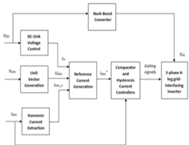
Fig. 2. Control Strategy Block.
