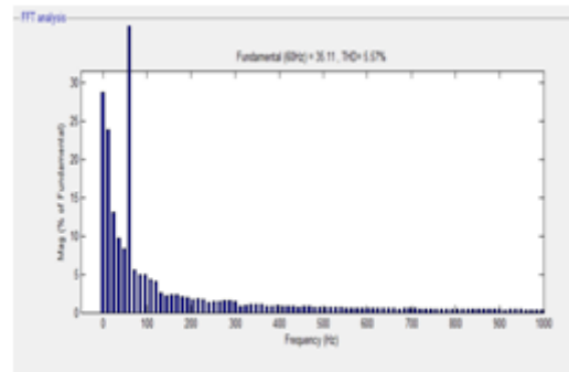
Fig. 12. FFT Analysis using Harmonic Extraction Method
