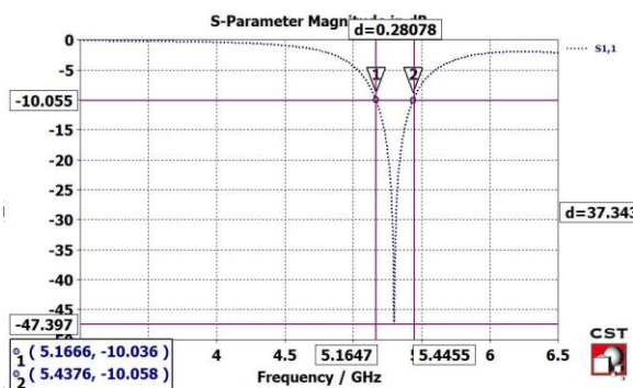
Figure 4: Bandwidth plot
