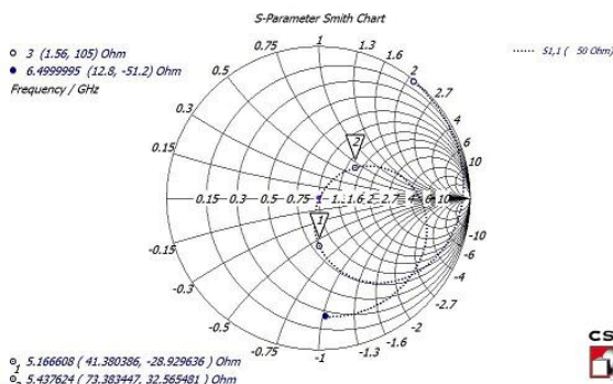
Figure 5: Curve showing antenna characteristic impedance
