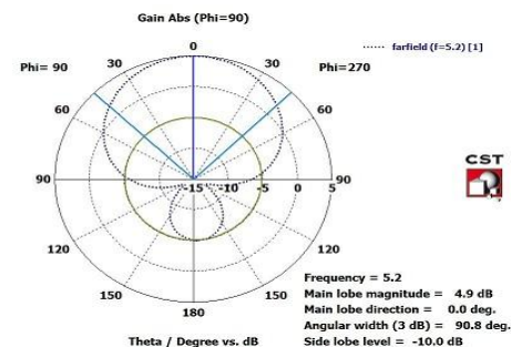
Figure 8: Gain of designed antenna
