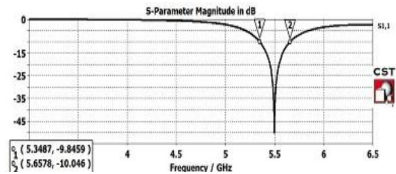
Figure 3: Stimulated return loss curve
