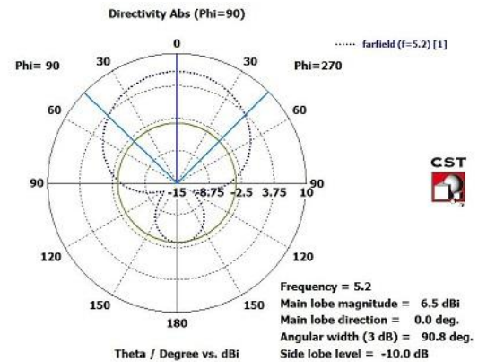
Figure 7: Directivity of designed antenna
