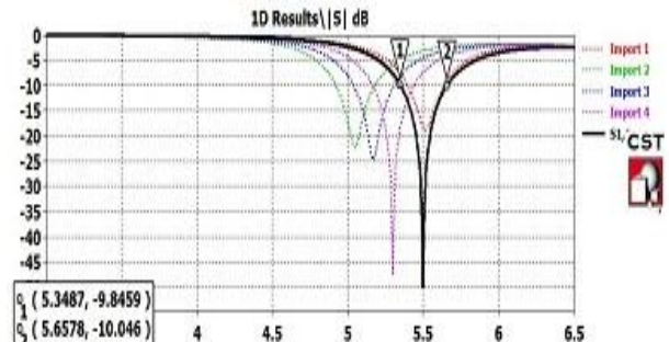
Figure 4: Stimulated return loss curve for different dimensions of defected ground H – shape
