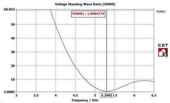
Figure 6: VSWR curve
